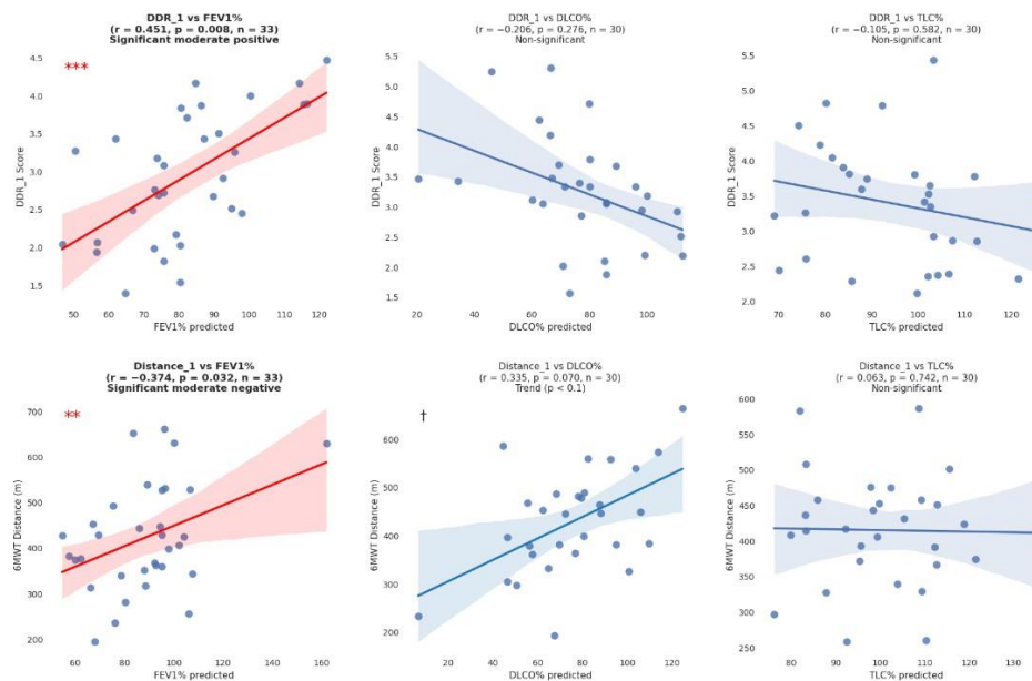
Figure 2: Correlation of DDR1 with PFT
